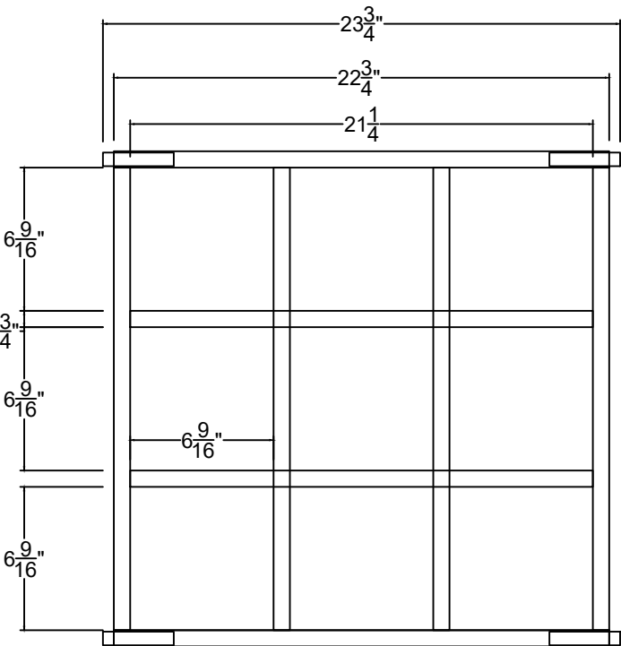
PLAN VIEW
