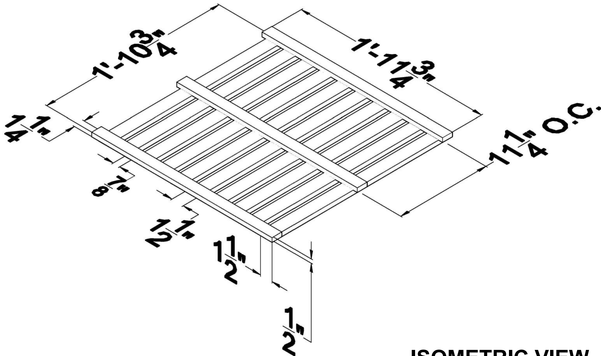
ISOMETRIC VIEW
