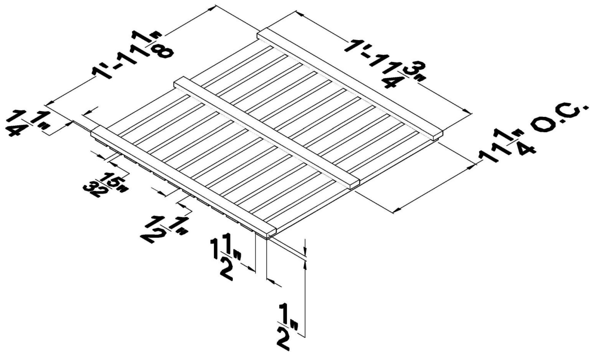
ISOMETRIC VIEW
