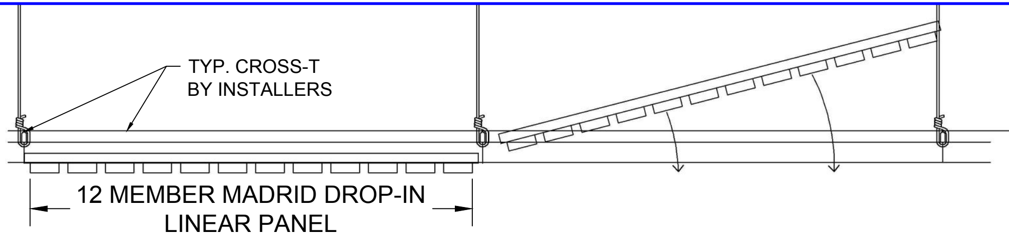
TYP. TEGULAR DROP-IN PANEL - INSTALLATION
