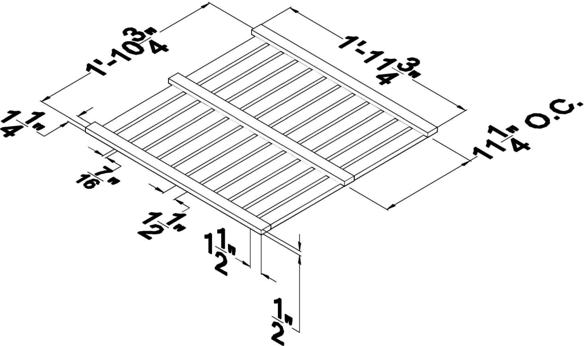
ISOMETRIC VIEW
