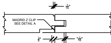
CONNECTION VIEW
