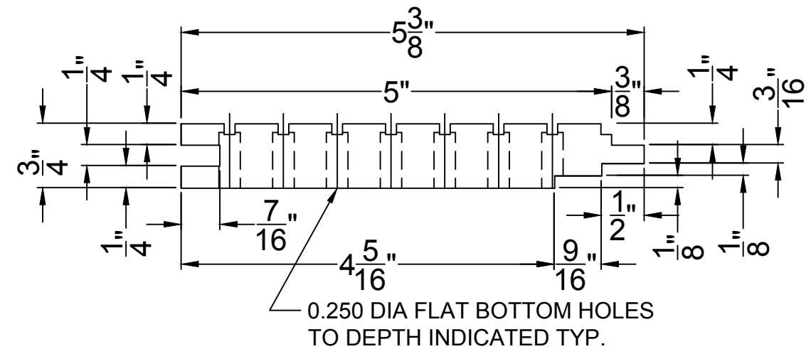
DETAIL A
