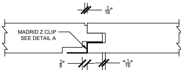
CONNECTION VIEW
