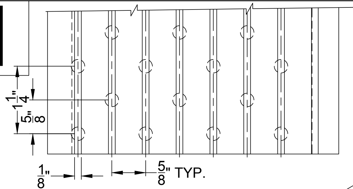
PARTIAL PLAN VIEW
