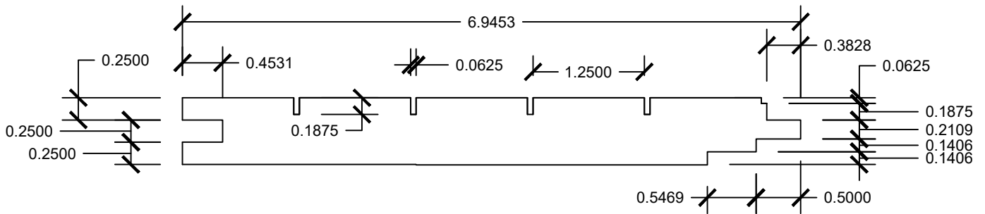
SIDE SECTION
