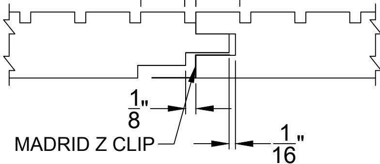
CONNECTION VIEW
