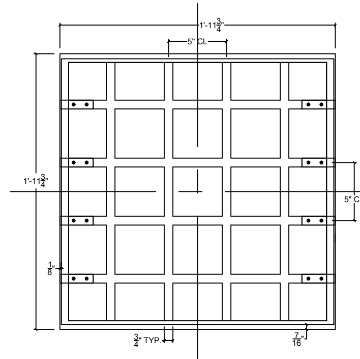
PLAN - 5" GRID LOCK
