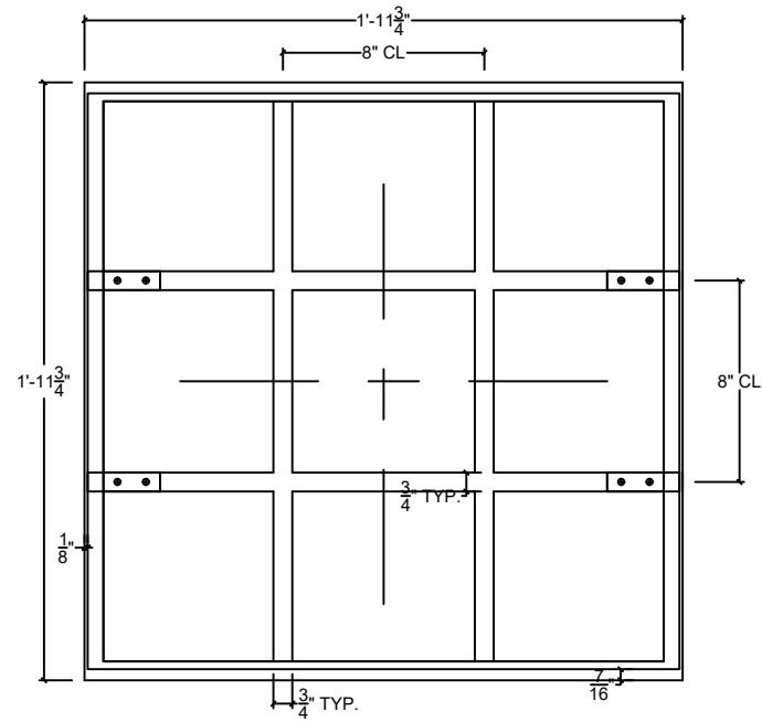
PLAN - 8" GRID LOCK
