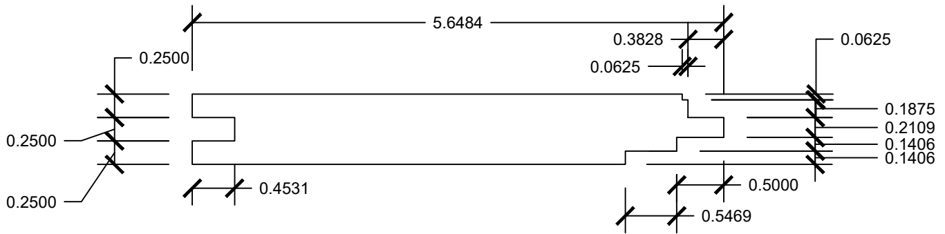
SIDE SECTION
