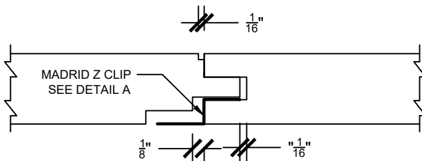
CONNECTION VIEW
