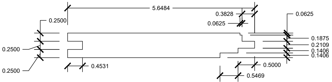
SIDE SECTION
