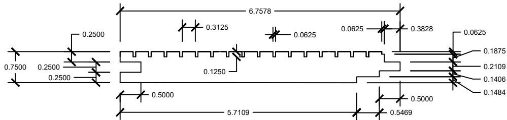
SIDE SECTION
