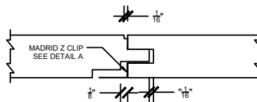
CONNECTION VIEW
