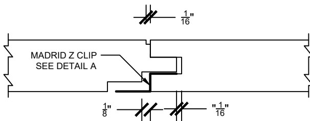
CONNECTION VIEW
