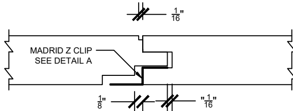
CONNECTION VIEW
