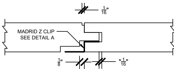
CONNECTION VIEW
