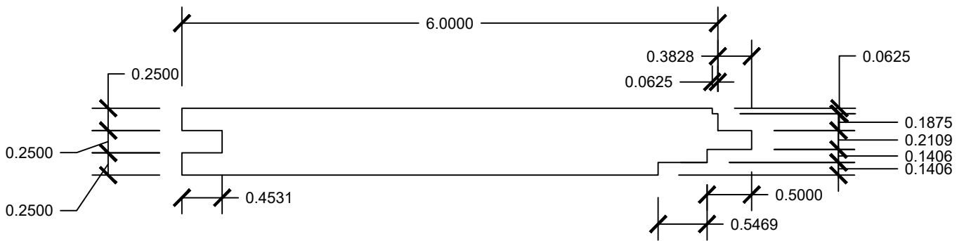
SIDE SECTION
