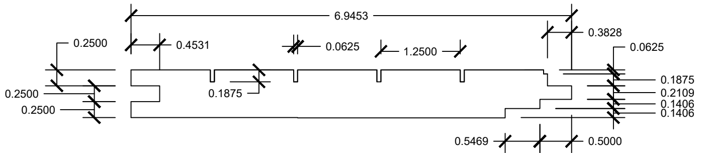
SIDE SECTION
