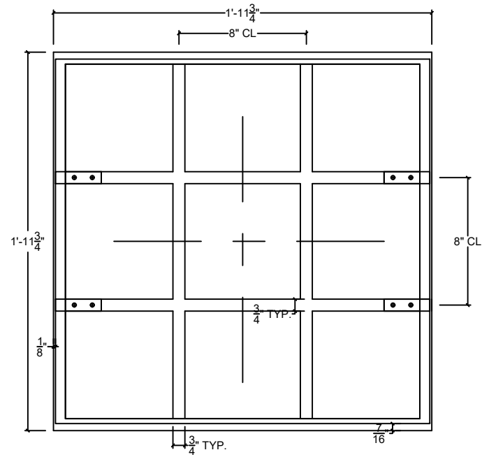
PLAN - 5" GRID LOCK
