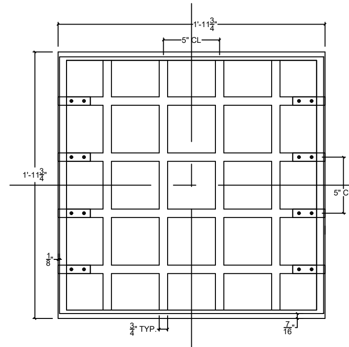
PLAN - 8" GRID LOCK
