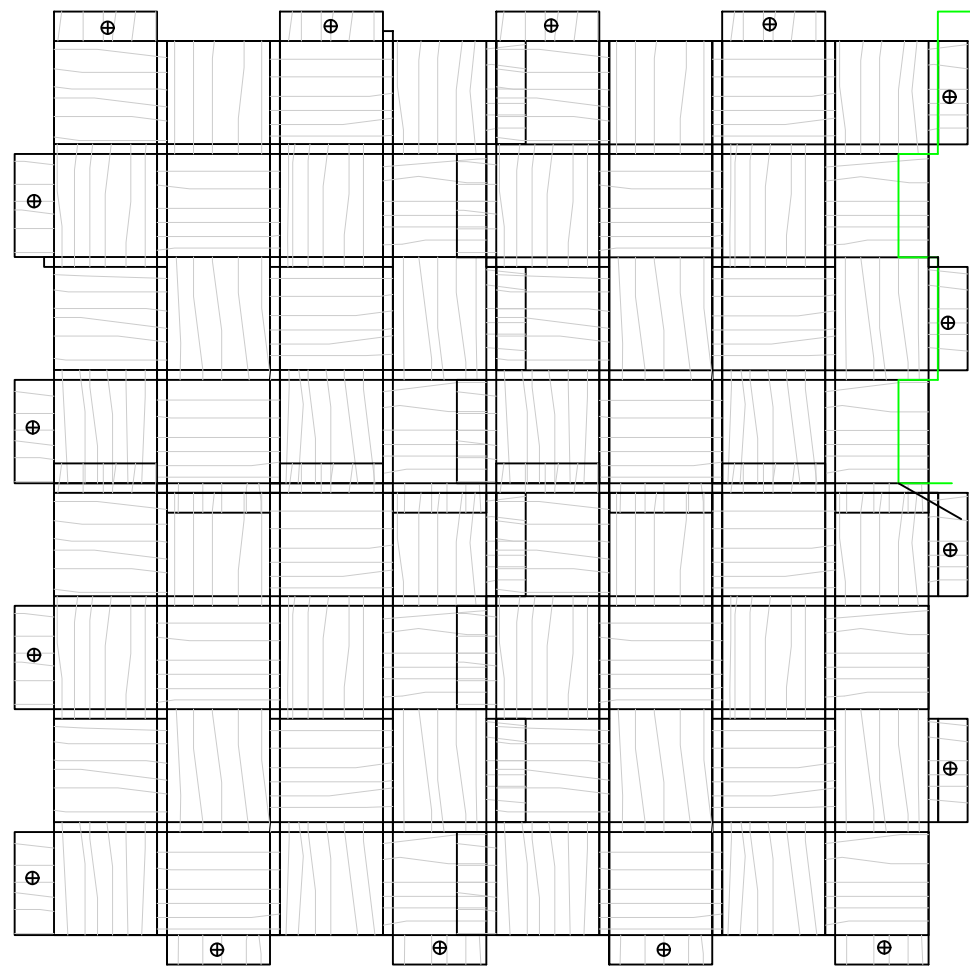
TYP. WALL INSTALLATION OF WOOD WEAVE PANELS
