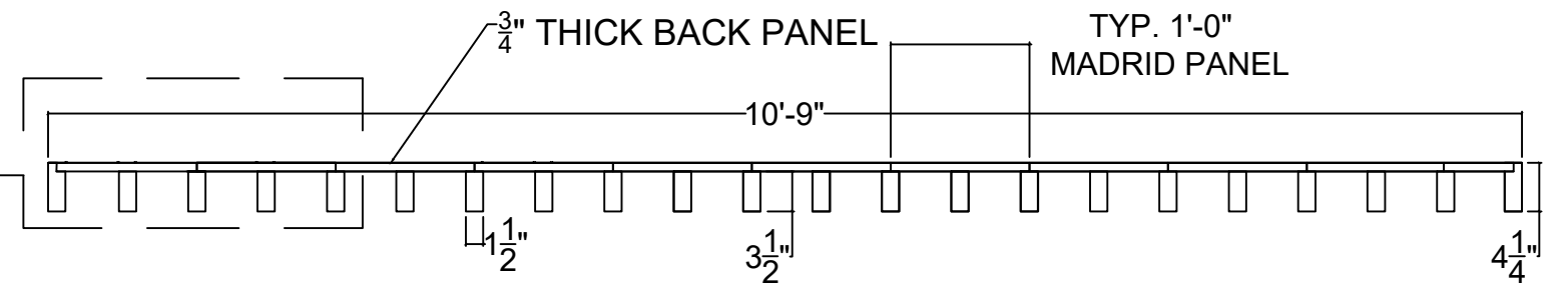
SIDE ELEVATION VIEW
