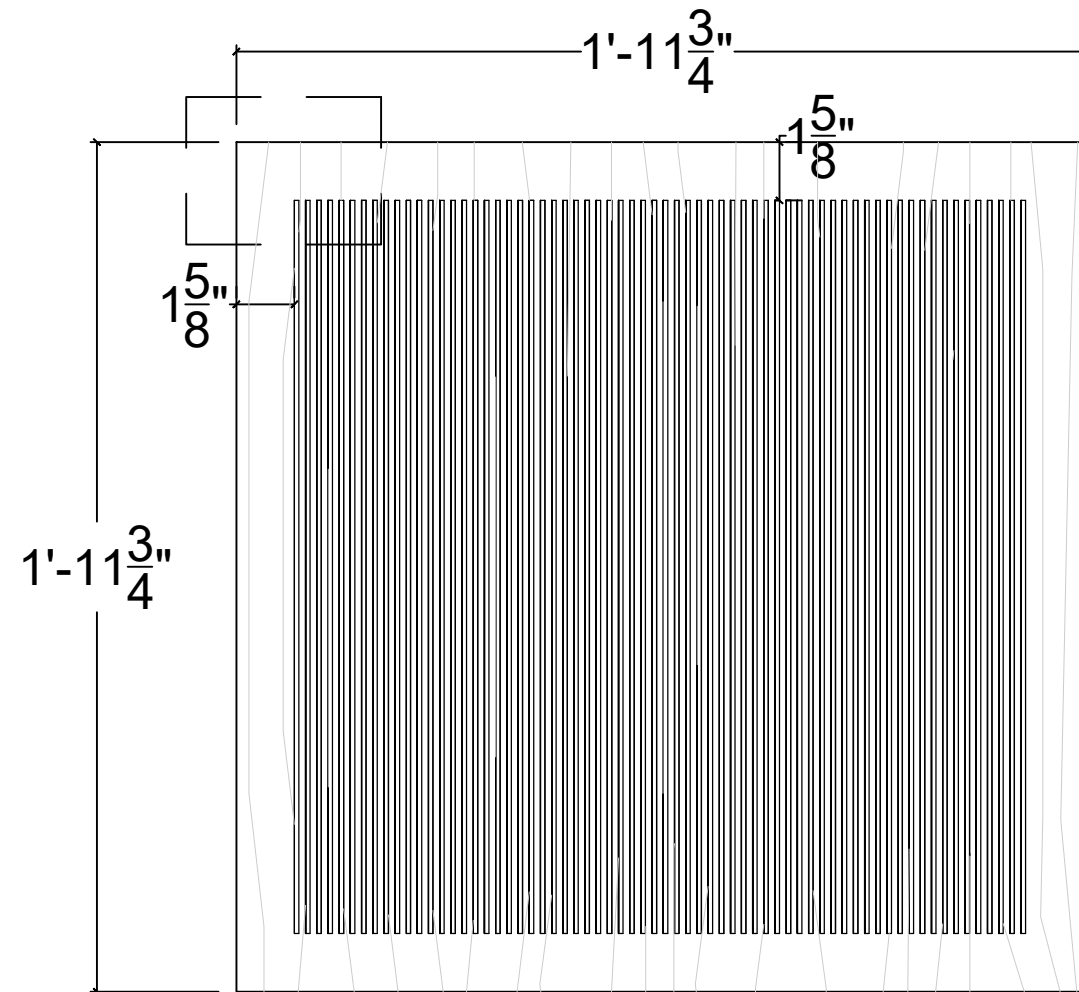
ENLARGED DETAIL
