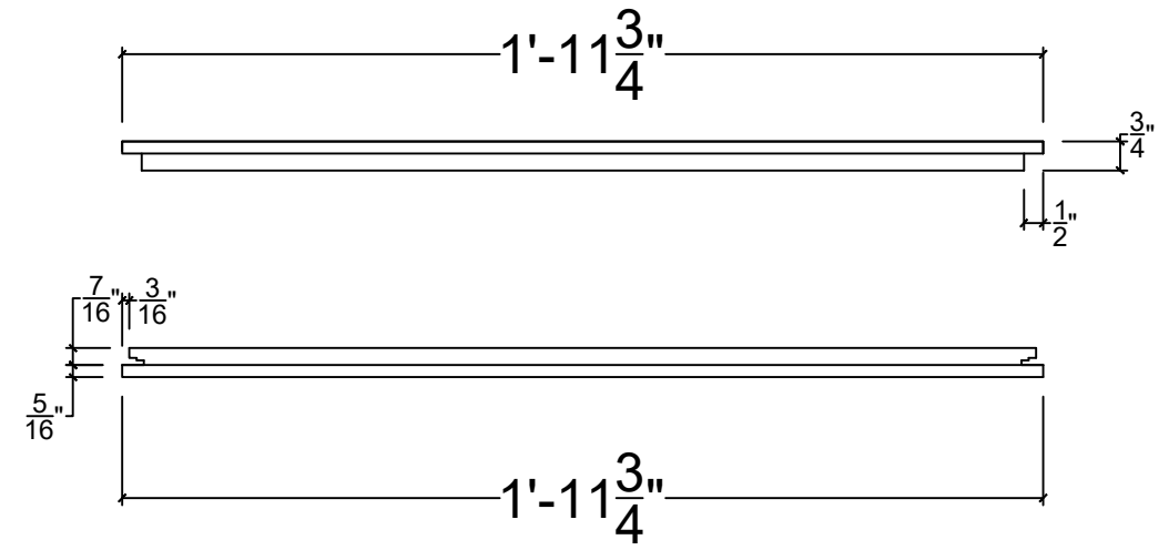
ELEVATION DETAIL
